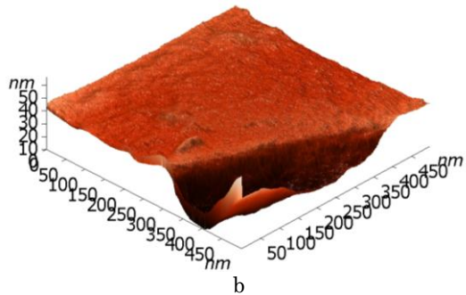
Fig. 5 – AFM topography of the non-coated textile samples (a) and 3D image (b)
