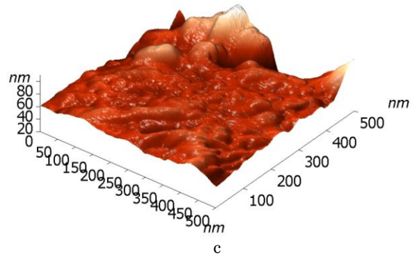
Fig. 6 – AFM topography of the coated textile samples zinc acetate concentration 2,5 %, dipping time 10 minutes (a), (b) and 3D image (c)
